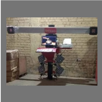
Unialiner 3D Wheel Alignment Machine
